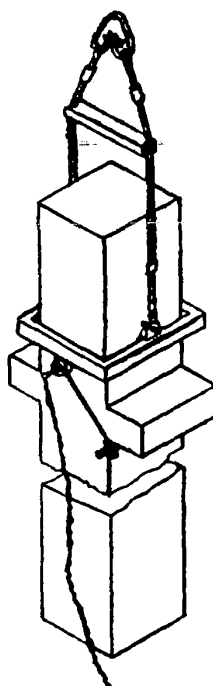
Строп 2СК-5,0 Q = 5,0 тс
